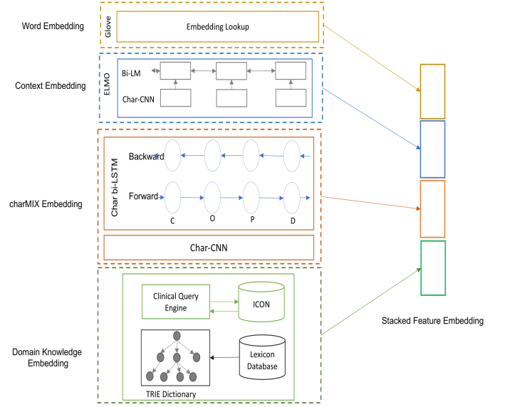
Fig. 2: Feature Representation
